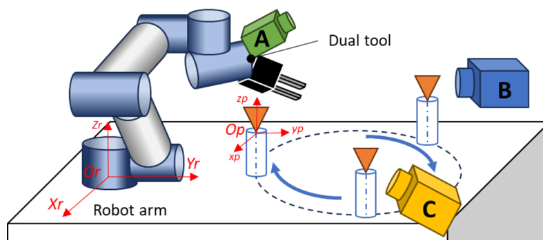
Fig.1 Work cell layout
