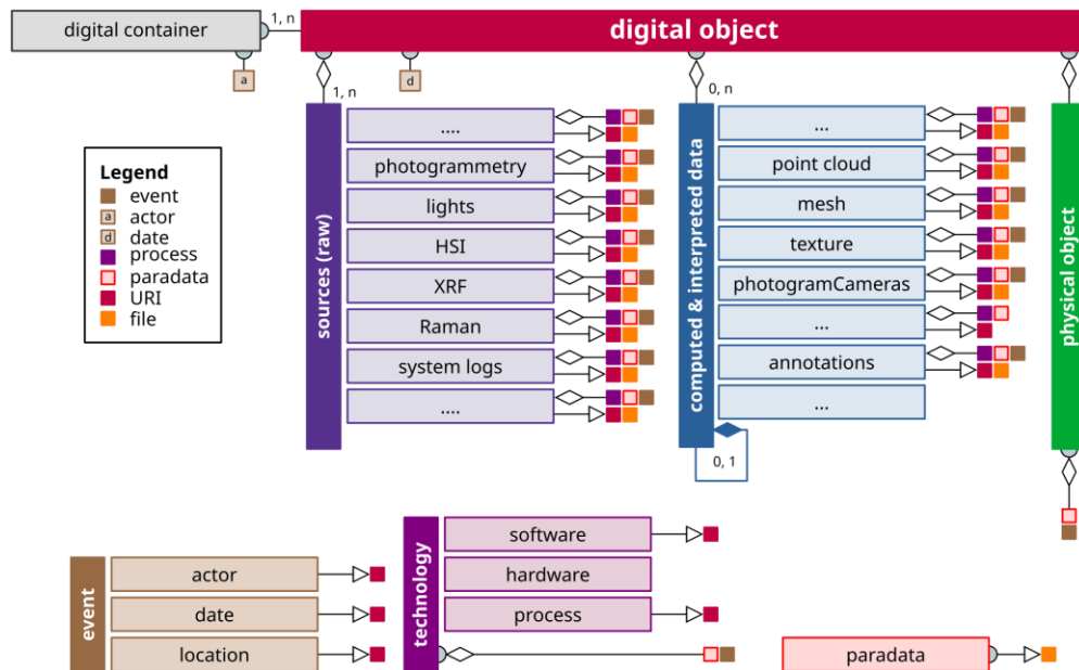
Fig. 1. Graphical overview of the required metadata for the AUTOMATA project, considering the use of photogrammetry for 3D creation, inspired by Quantin et al. (2025). Each block will be detailed in the document. 1,n stands for at least one element, while 0,n indicates that the number is free. 1 indicates that a unique element is mandatory.
